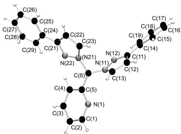
Figure 2. Molecular structure of L4 .
