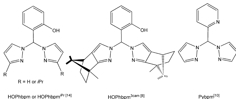
Figure 1. Classical members of the bis(pyrazolyl)methane family.
