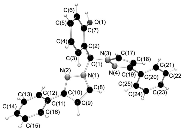
Figure 3. Molecular structure of L6 .
