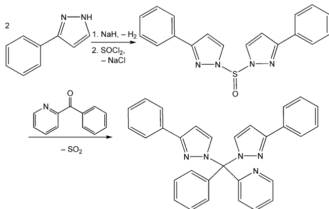
Scheme 3. Synthesis of L13 .
