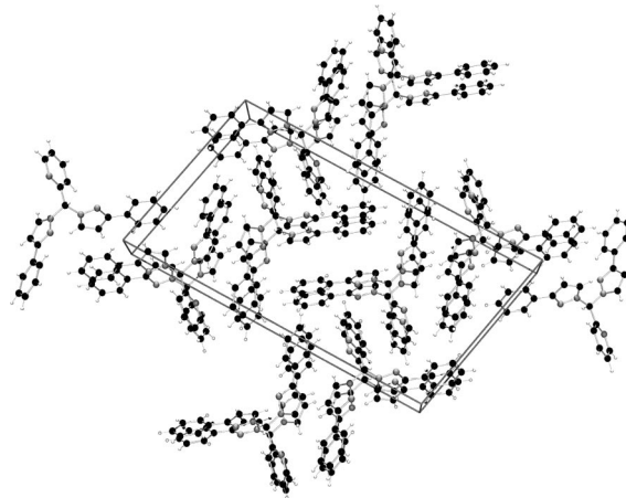
Figure 4. Crystal packing of L4 .
