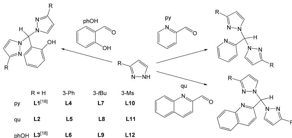
Scheme 2. Overview of the synthesized ligands. [18]
