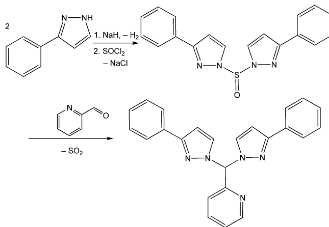
Scheme 1. Synthesis of L4 .
